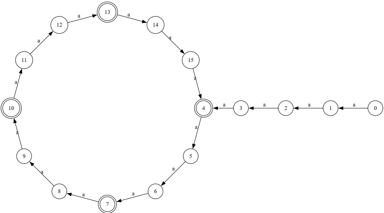
Figure 2. Example md-DFA for the expression “ ((aaaa)^*a\{1,4\})\{4000\}-(a\{1,3\}(aaa)^*)\{4000\} ”.
