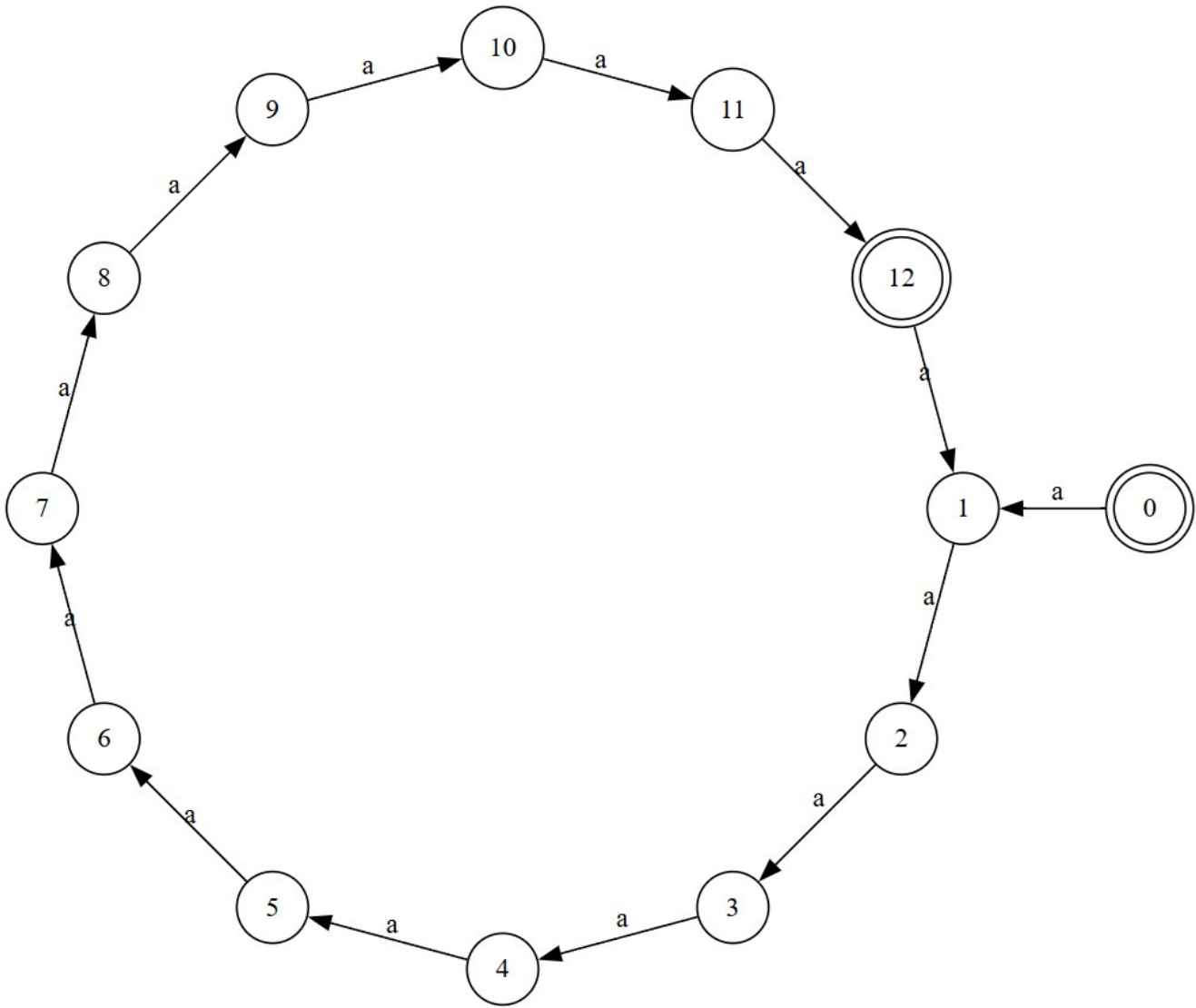
Figure 6. The non-emptiness DFA for the expression “((a)*)&((aa)*)&((aaa)*)&((aaaa)*)&((aaa)*)”.
