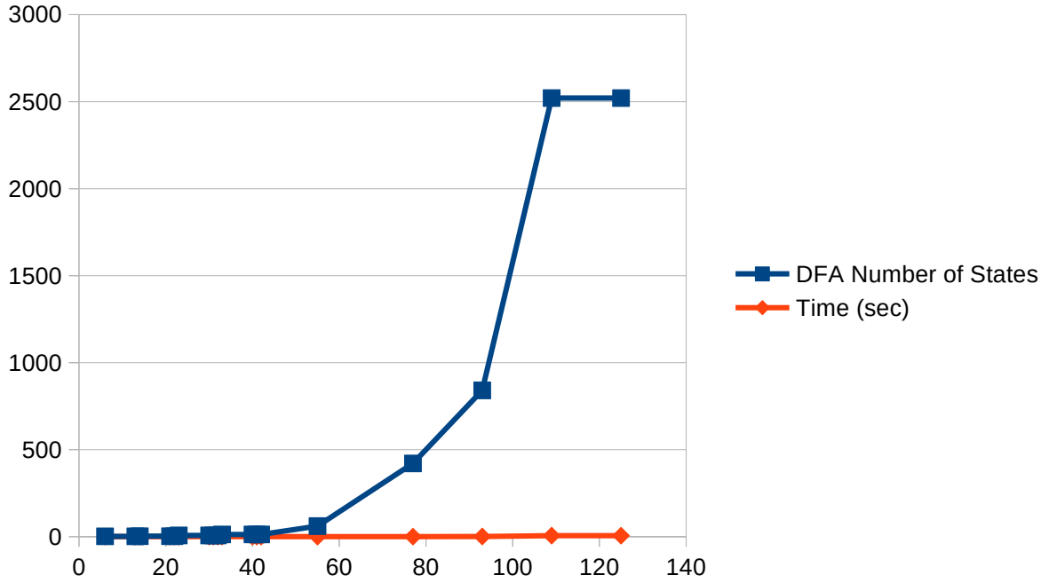
Figure 5. The visualization of the performance of the non-emptiness test algorithm.
