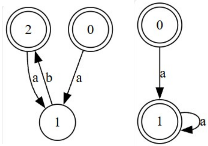
Figure 7. The resulting DFAs for expressions “((ab)*)&...” and “(a*a)&...”
