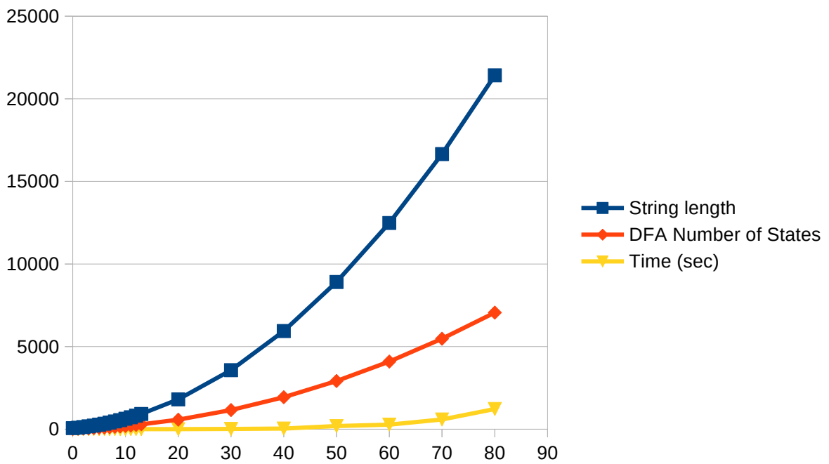
Figure 3. Visualization of the benchmarks in Table 2.
