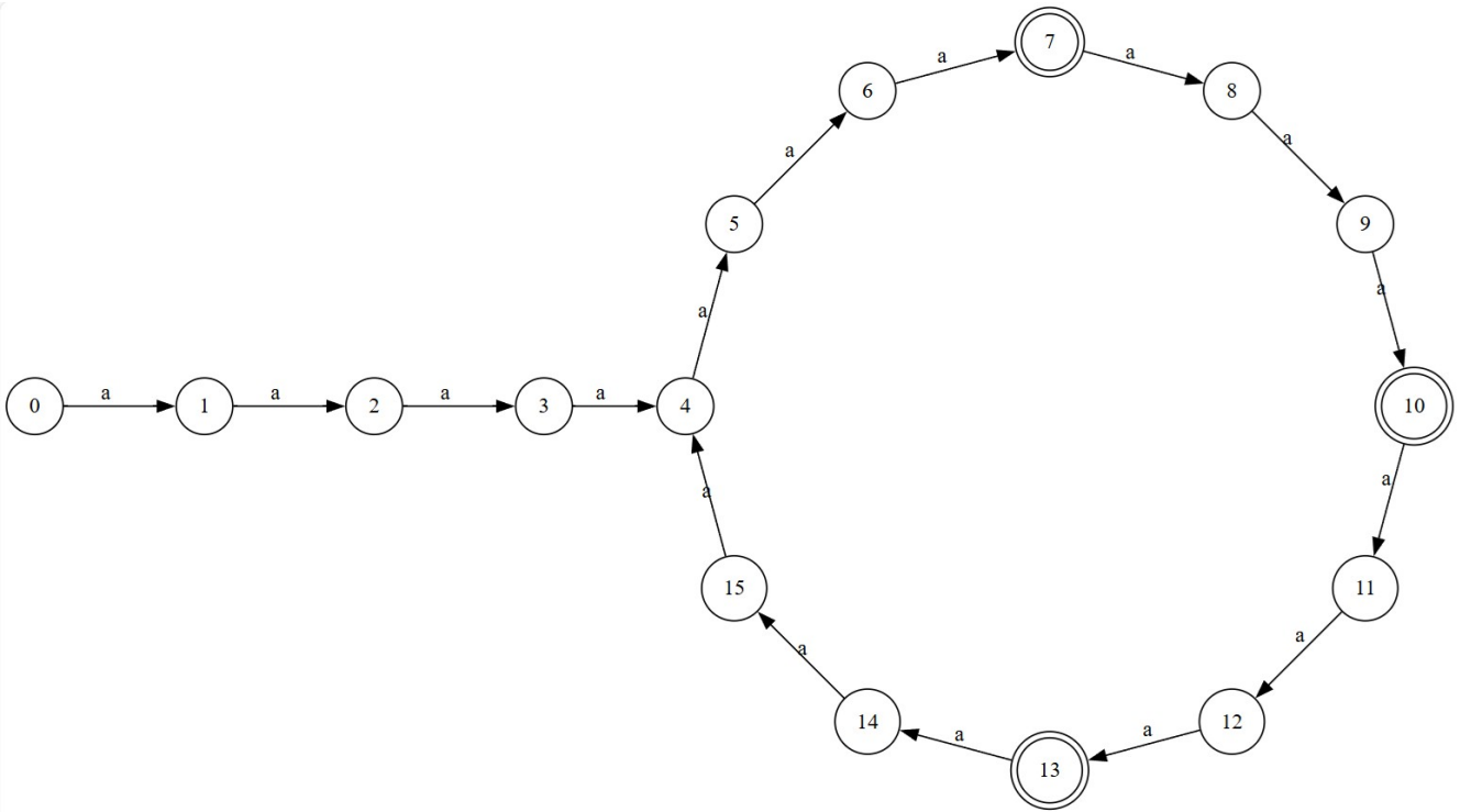
Figure 1. The distinguishing DFA for example in [5].
