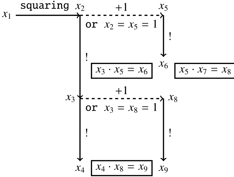
Fig. 3 Construction of the system \mathcal{A}
