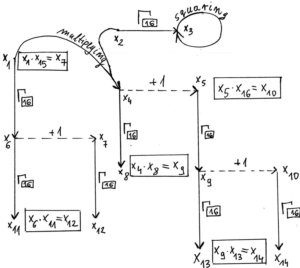
Fig. 9 Construction of the system Z_{16}
