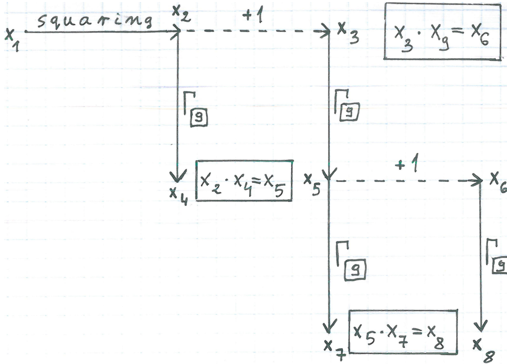
Fig. 7 Construction of the system \mathcal{Z}_9
