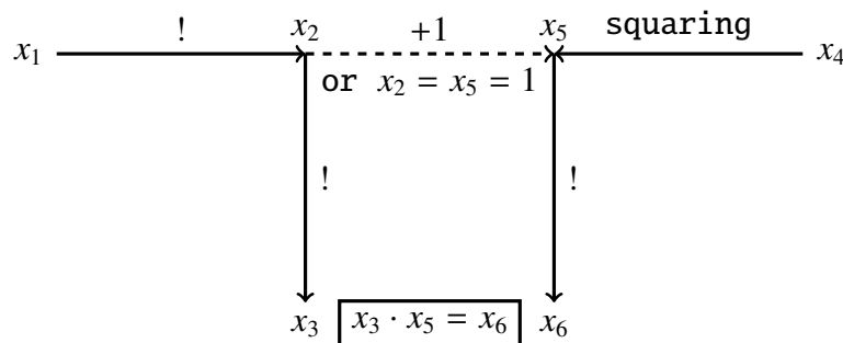
Fig. 3 Construction of the system \mathcal{A}
