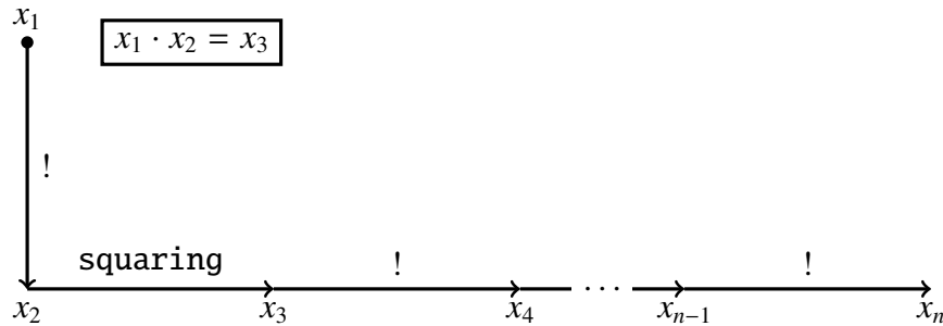
Fig. 2 Construction of the system \mathcal{U}_n
