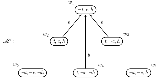
Figure 17: Model resulting from revising the model \mathcal{M} in Figure 15 with the new effect law token \rightarrow [buy]\neg token .
