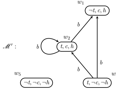
Figure 16: Model resulting from revising the model \mathcal{M} in Figure 15 with \neg\text{coffee} \rightarrow \neg\text{hot} .
