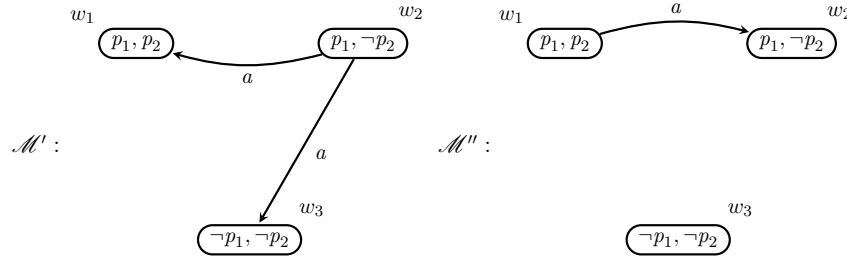
Figure 11: Models resulting from contracting p_1 \rightarrow \langle a \rangle \top in the model \mathcal{M} of Figure 10.
