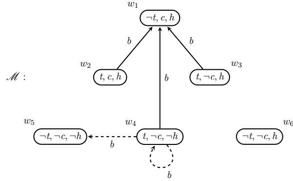
Figure 7: Two candidate new buy -arrows to falsify token \rightarrow [buy]hot in \mathcal{M} .
