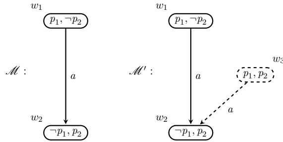
Figure 12: Adding a transition from a new added world in the alternative semantics to static law contraction. \mathcal{M} denotes the original model, while \mathcal{M}' shows the new added world and a candidate transition to add to R_a .
