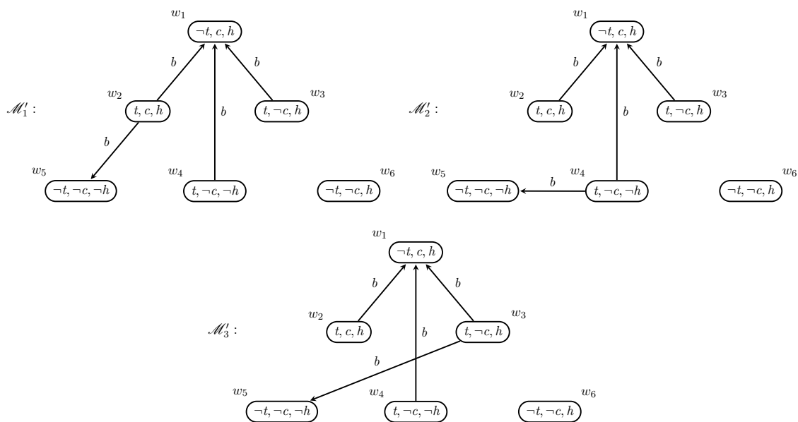
Figure 8: Models resulting from contracting token \rightarrow [buy]hot in the model \mathcal{M} of Figure 4.
