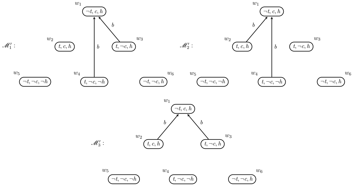
Figure 5: Models resulting from contracting token \rightarrow \langle buy \rangle \top in the model \mathcal{M} of Figure 4.
