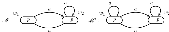
Figure 19: Counter-example to preservation in the method by Herzig et al. (2006).
