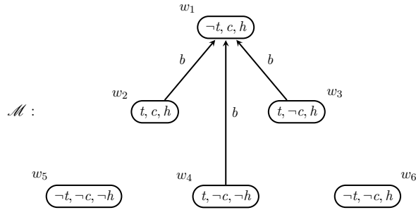
Figure 4: The canonical model for the coffee machine scenario.
