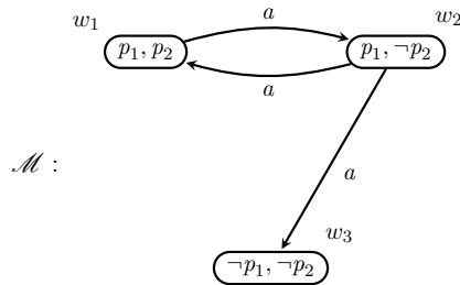
Figure 10: A model of the executability law p_1 \rightarrow \langle a \rangle \top .
