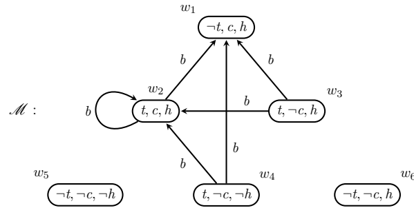
Figure 15: Canonical model of the new initial action domain description.
