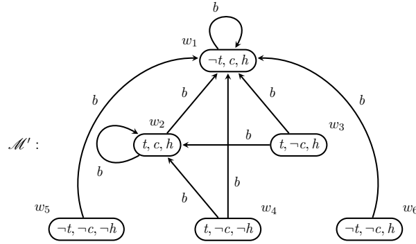
Figure 18: Result of revising \mathcal{M} in Figure 15 by the new executability law \neg token \rightarrow \langle buy \rangle \top .
