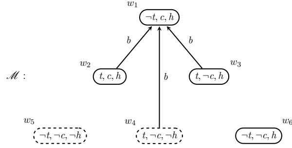
Figure 6: Candidate worlds to receive transitions coming from token -worlds.
