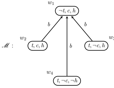
Figure 3: A model for our coffee machine scenario: b , t , c , and h stand for, respectively, buy , token , coffee , and hot .
