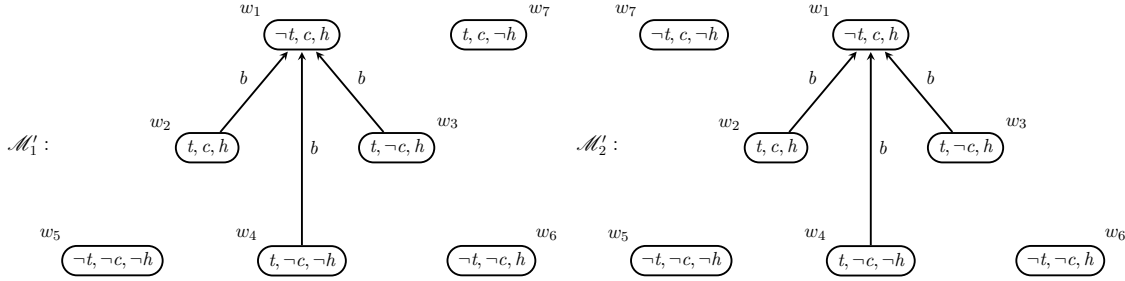
Figure 9: Models resulting from contracting coffee \rightarrow hot in the model \mathcal{M} of Figure 4.
