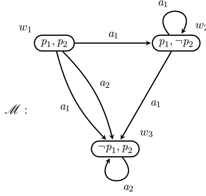
Figure 2: Example of a \mathcal{K}_n -model for \mathfrak{Act} = \{a_1, a_2\} , and \mathfrak{Prop} = \{p_1, p_2\} .
