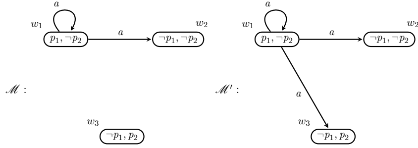
Figure 13: A model \mathcal{M} of \mathcal{T} and the result \mathcal{M}' of contracting p_1 \rightarrow [a]\neg p_2 in it.
