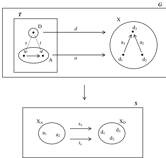
Figure 4: A graph morphism a : A \rightarrow X from an object A (in the theory T of the category G of graphs) to a graph X is an A -shaped figure in X , and a morphism d : D \rightarrow X is a D -shaped figure in X . The set of all morphisms from A to X is the set X_A of all arrows in X , and the set of all morphisms from D to X is the set X_D of all dots in X . Any morphism from A to X can be pre-composed with a morphism from D to A to obtain a morphism from D to X . Pre-composing an arrow a : A \rightarrow X with source s : D \rightarrow A gives a morphism from D to X , which is the source dot of the arrow a : A \rightarrow X ; pre-composing with target t : D \rightarrow A gives the target dot. Thus we obtain a parallel pair of functions s_x, t_x : X_A \rightarrow X_D , specifying for each arrow (in the set X_A of arrows) its source, target dot (in the set X_D of dots), as a model of the graph X in the category S of sets.
