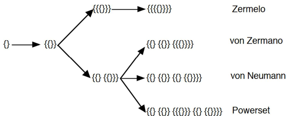
Figure 3. Beginnings of four minimal \omega -series
