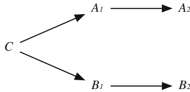
Fig. 2 Screening off without a common cause
