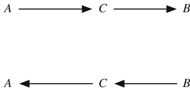
Fig. 2 Screening off without a common cause
