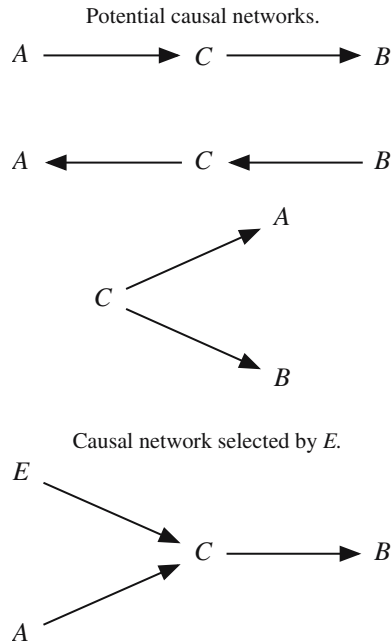
Fig. 4 Fixing temporal orientation with further probabilities
