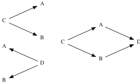
Fig. 1 Open and closed forks
