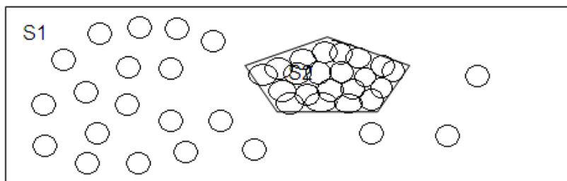
Figure 7: S2 covered by circles of radius r
