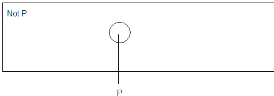
Figure 2: P is a positive proposition
