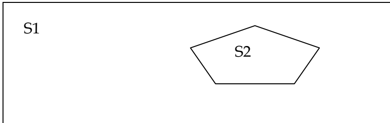
Figure 6: S1 is greater than S2
