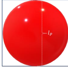
Figure 6. The smallest geometry in the Universe is the Planck Area, here illustrated as a sphere. The corresponding Z-Planck is given by Eq. 28.
