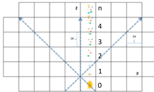
Figure 2. ITP says that if the whole spacetime is finite, then it could be divided so that each resulting segment could be thought of as time. This means that no internal elements could move out between two temporal levels. Each level of time corresponds to one universal space-like surface or the current Universe. Note also that light only moves forward along with time segments.
