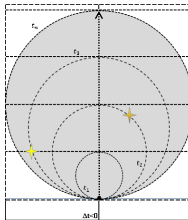
Figure 3. Relative to an external observer, the Universe contains static equitemporal contours (isometric lines) – setting boundaries between each segment that contains unique configurations in spacetime. Each static isocurve (contour) is globally equitemporal. The Universe U has a proper time, assuming ITP to be true.
