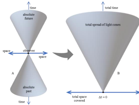
Figure 4. (A) The Universal Light Cones (i.e., the two nappes being equal) are the path that a flash of light, emanating from a single event (i.e., the Big Bang singularity at the center), travels in all directions. (B) The total light spread from beginning to end – covering the entire history of the Universe.
