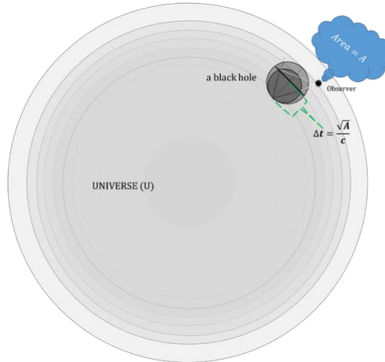
Figure 8. A simplified side view of the static 4D Universe hosting a black hole – a possibly micro-universe itself. We could estimate the time for the blackhole's Schwarzschild radius to reach its size by simply dividing its diameter by c (see Eq. 45). Notice that the origin of the black hole is depicted to originate below its observed area A just like the Universe that has its point of beginning relative to internal observers.
