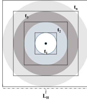
Figure 5. The possible suggestions of the Z-energy flux rate with the side of the frame equal to the Hubble Length (i.e., the Z-Hubble, see Eq. 44). Could Z be describing a pixel or a projector where energy diffusion flux occurs? The view here is eye-level with the arrow of time towards the viewer. Also notice that temporal gradations are enclosed. The time-like, static Universe is made up of multi-layered shells of space-like contemporaneous Universes of time t_1 , t_2 , up to t_n .
