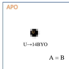
Figure 10. APO timelessly contains U. If U is wrinkled and since APO is smooth and simple, APO must be timeless and processless. Notice that APO is not sequential to be A+B and U is eternally wrinkled as ~14 billion years old (i.e., 14 billion 1-sec static gradation) because the contours are invariant or increasing.
