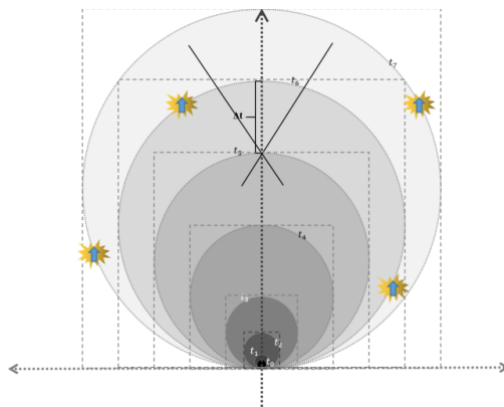
Figure 7. Top view: The Universe is ballooning with time where each circular line is equitemporal. Quantum entanglement may be an equitemporal form of communication (i.e., always along the equitemporal line, say, t_4 ) that does not travel between or at an angle with the time-like direction.
