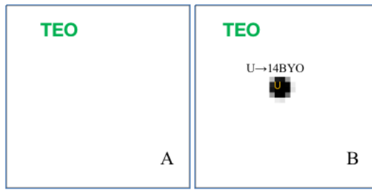
Fig. 9. The usual assumption for the Universe: TEO at (A) pre- and (B) post-appearance of U of age 14 billion years old (BYO). The point-sized Universe U is exaggerated in B for emphasis. The immense TEO is illustrated as the larger square for simplicity.
