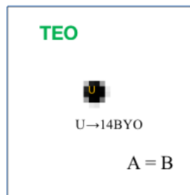
Fig. 10. TEO timelessly contains U. If U is wrinkled and since TEO is smooth and simple, TEO must be timeless and processless. Notice that TEO is not sequential to be A+B and U is eternally wrinkled as \sim 14 billion years old (i.e., 14 billion 1-sec static gradation) because the contours are invariant or increasing.
