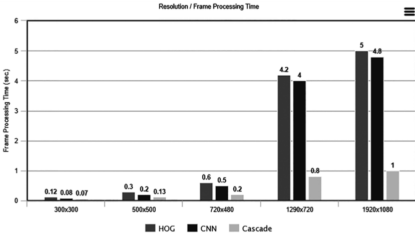
Fig. 9 Input video resolution / frame processing time relationship for the HOG, CNN and the Haar Cascade algorithms
