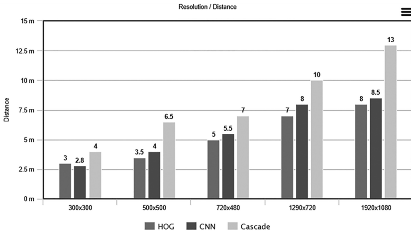
Fig. 8 Input video resolution / maximum face distance from the camera relationship for the HOG, CNN and the Haar Cascade algorithms
