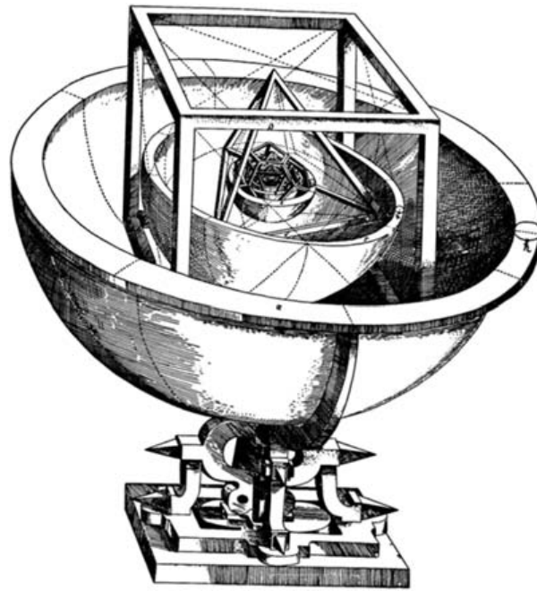
Figure 1 Kepler's model of solar system (Kepler 1981 [1596])
