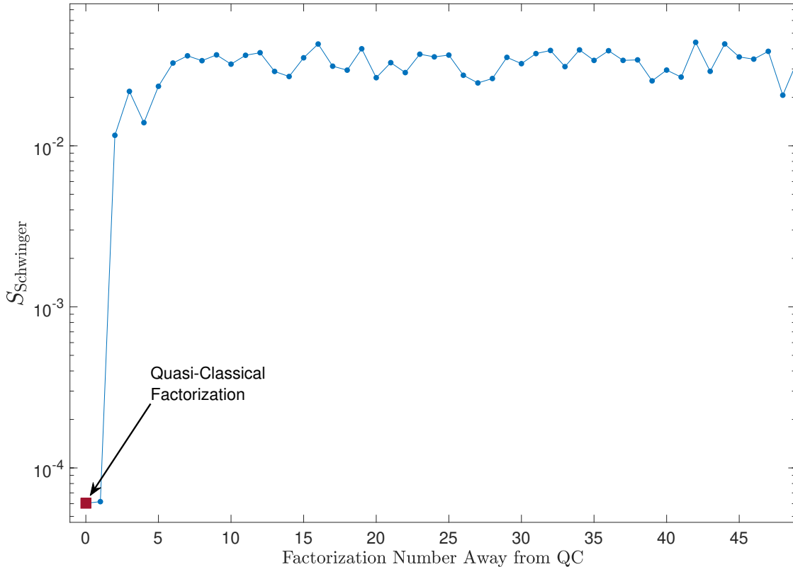
FIG. 6: Quantum Mereology Algorithm: a run similar to figure 5 sifting through different factorizations of Hilbert space but this time with larger, successive perturbations away from the identity operator to generate the unitary transformation \Lambda . In the QC factorization, which minimizes the Schwinger entropy, the quantum system is described by two harmonic oscillators coupled by their positions. Factorizations away from QC quickly saturate to generic, large values of Schwinger entropy. The quasi-classical factorization (the first factorization we begin with) is marked by a red square. Details in the text.
