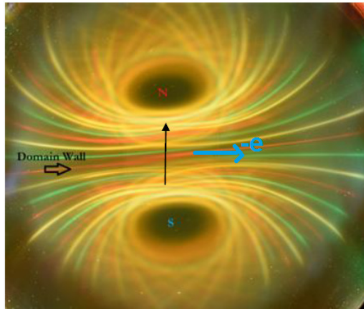
Figure 2. Domain wall inside the electron (After Markoulakis)
