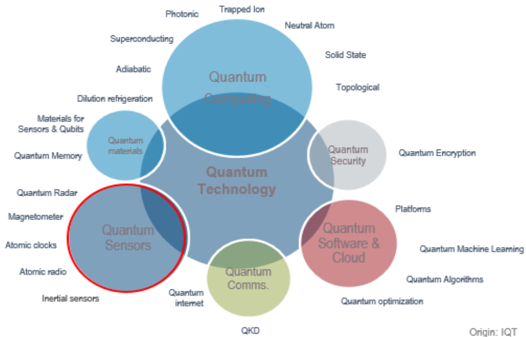
Figure 1. Quantum disciplines (modified from an original In-Q-Tel diagram).
