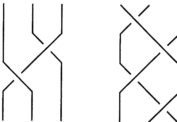
FIGURE 1. Two 3-stranded braids
