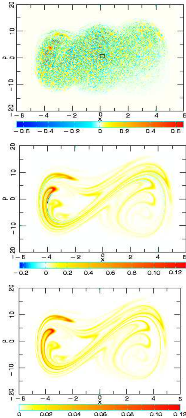
Figure 1. Top: solution of (2) with time t = 8T , where T is the period of the driving force, D = 0 , quantum interference with no decoherence. Middle: solution of (2) with t = 8T , D = 0.025 , decoherence suppresses quantum interference. Bottom: solution of (3), t = 8T , D = 0.025 , classical distribution. [Habib et al. (1998)].
