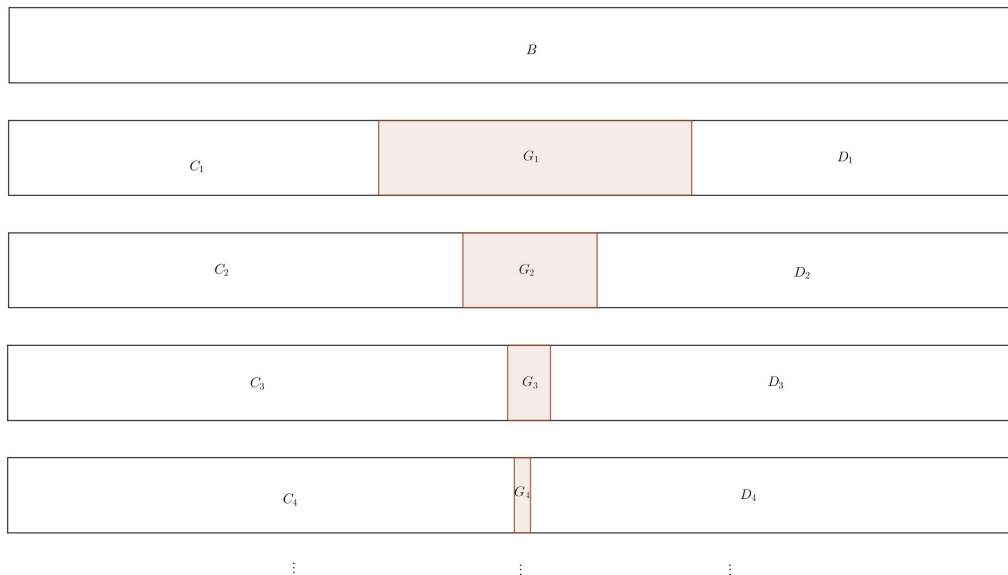
Figure 3.1: Savage's error reducing partitions
