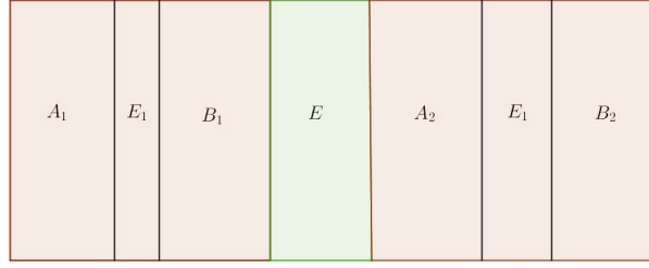
Figure 3.3: Claim in the proof of Theorem 3.17
