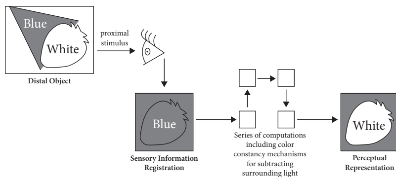
C4F1 Figure 4.1 An idealized model of seeing a red berry under blue light.
