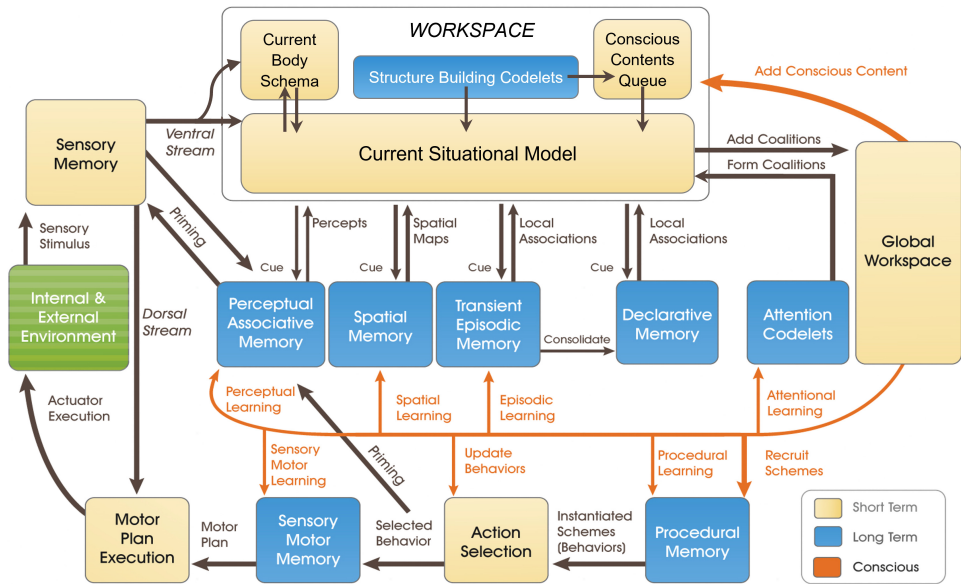
Fig. 3. Schematic of the LIDA cognitive architecture.
