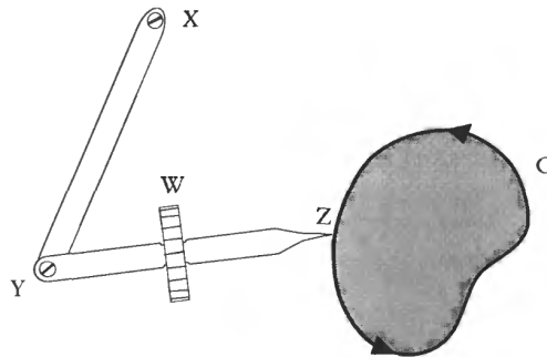
Figure 2: Polar planimeter. From Jennings (1994, 39).
