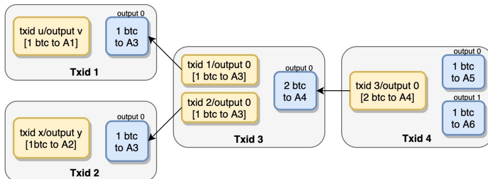
Figure 7. The transactions in Figure 6, with inputs and outputs.
