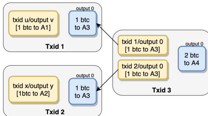
Figure 5. The inputs and outputs from transactions in Figure 4.
