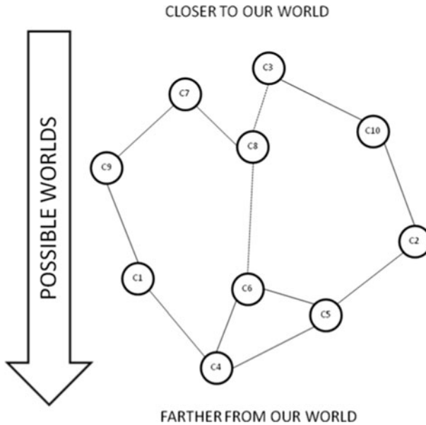
Fig. 2 Illustration of the Wright-Fisher Model as a network of ideal conditions of different degrees of idealization
