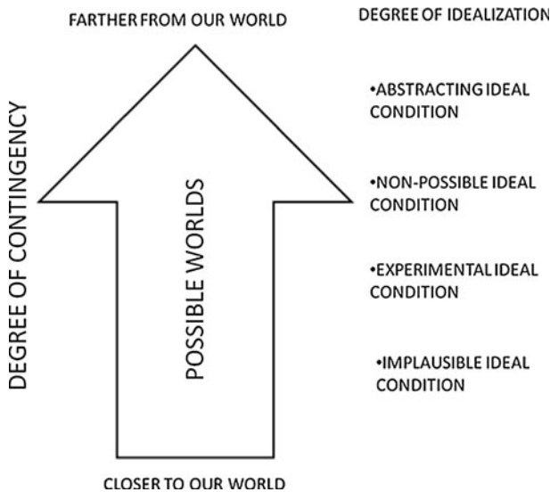
Fig. 1 Diagram representing the degree of idealization for different idealized conditions according to their distance from the actual world
